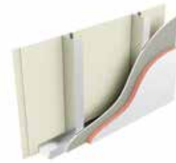
Type E2: Two layers of plasterboard, stud, sheathing board, 50mm K15 Insulation
