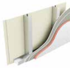
Type E3: Two layers of plasterboard, stud, two layers of sheathing board, 50mm K15 Insulation
