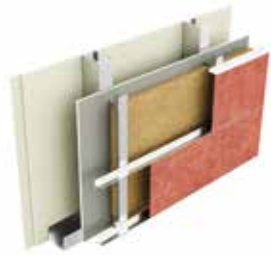
Type EC2: Two layers of plasterboard, stud, sheathing board, insulation, ventilated rainscreen
