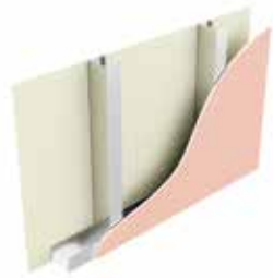
Type H1: Layer of plasterboard, stud, layer of plasterboard
