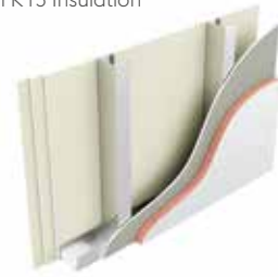
Type LE6: Three layers of plasterboard, stud, sheathing board, 50mm K15 Insulation
